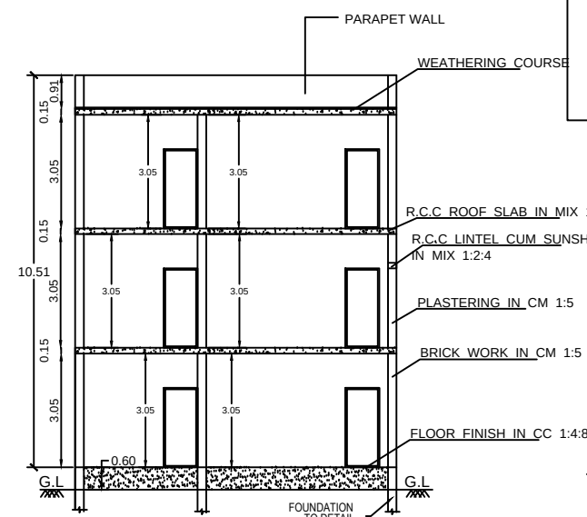
SECTION ON-'AB'
