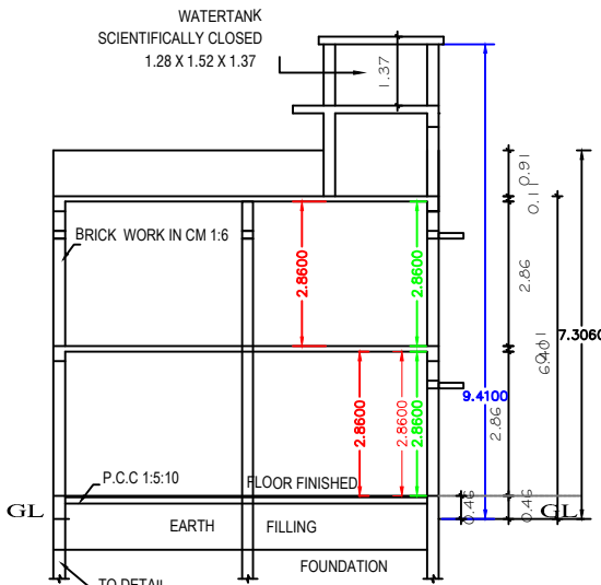
SECTION "A-B"
