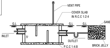
SECTION-AB
