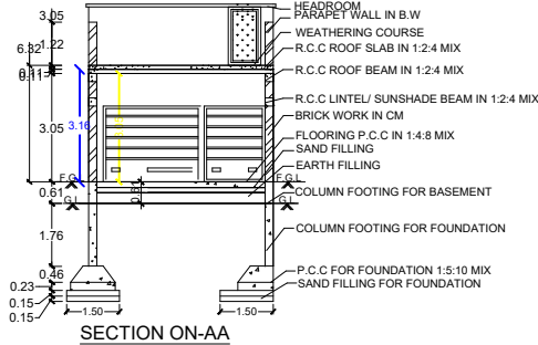
SECTION ON-AA
