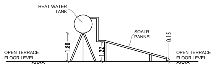
SIDE ELEVATION
