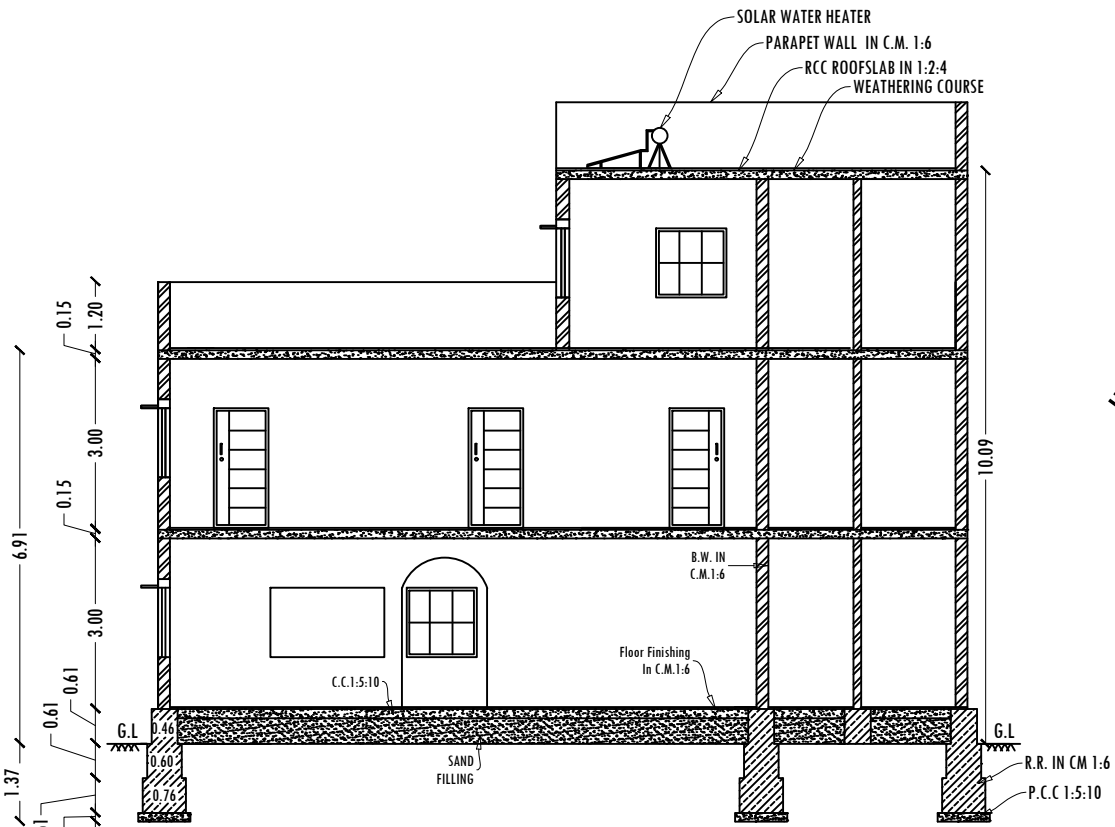
SECTION -AA
