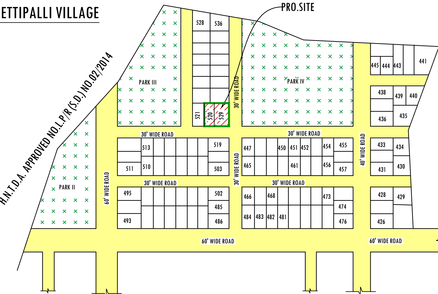
LOCATION PLAN
