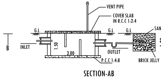
SECTION-AB
