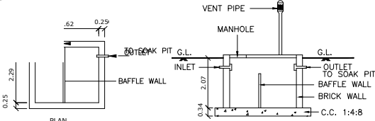
SECTION OF SEP.TANK
