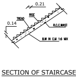
SECTION OF STAIRCASE
