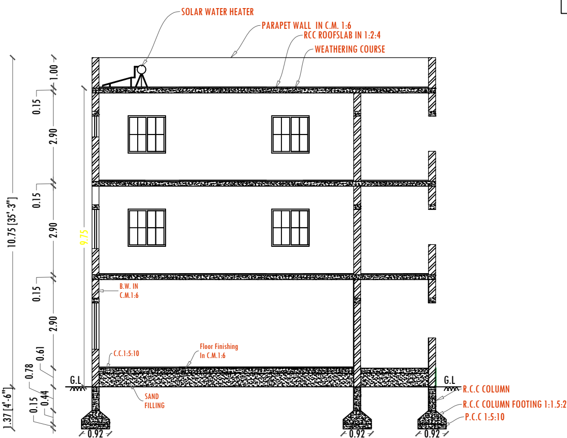
SECTION -AA
