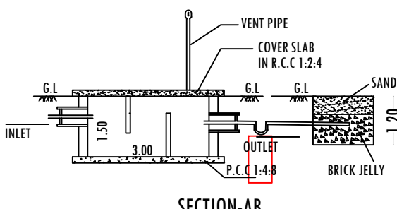
SECTION-AB
