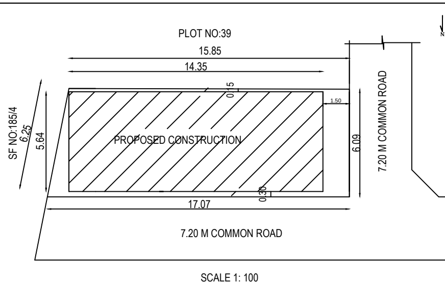
SCALE 1: 100
