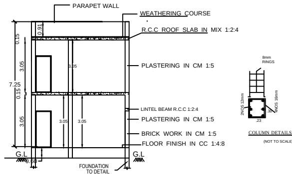
SECTION ON-"AB"
