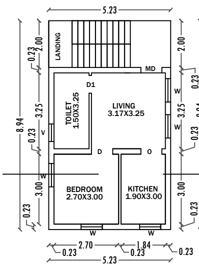
FIRST FLOOR SCALE:1:100
