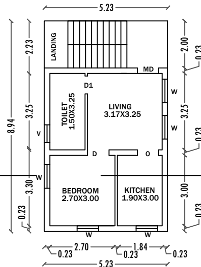
SECOND FLOOR SCALE:1:100
