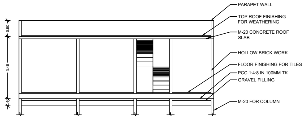
CROSS SECTION
