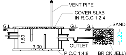
DETAILS OF RAIN WATER HARVESTING STRUCTURES
