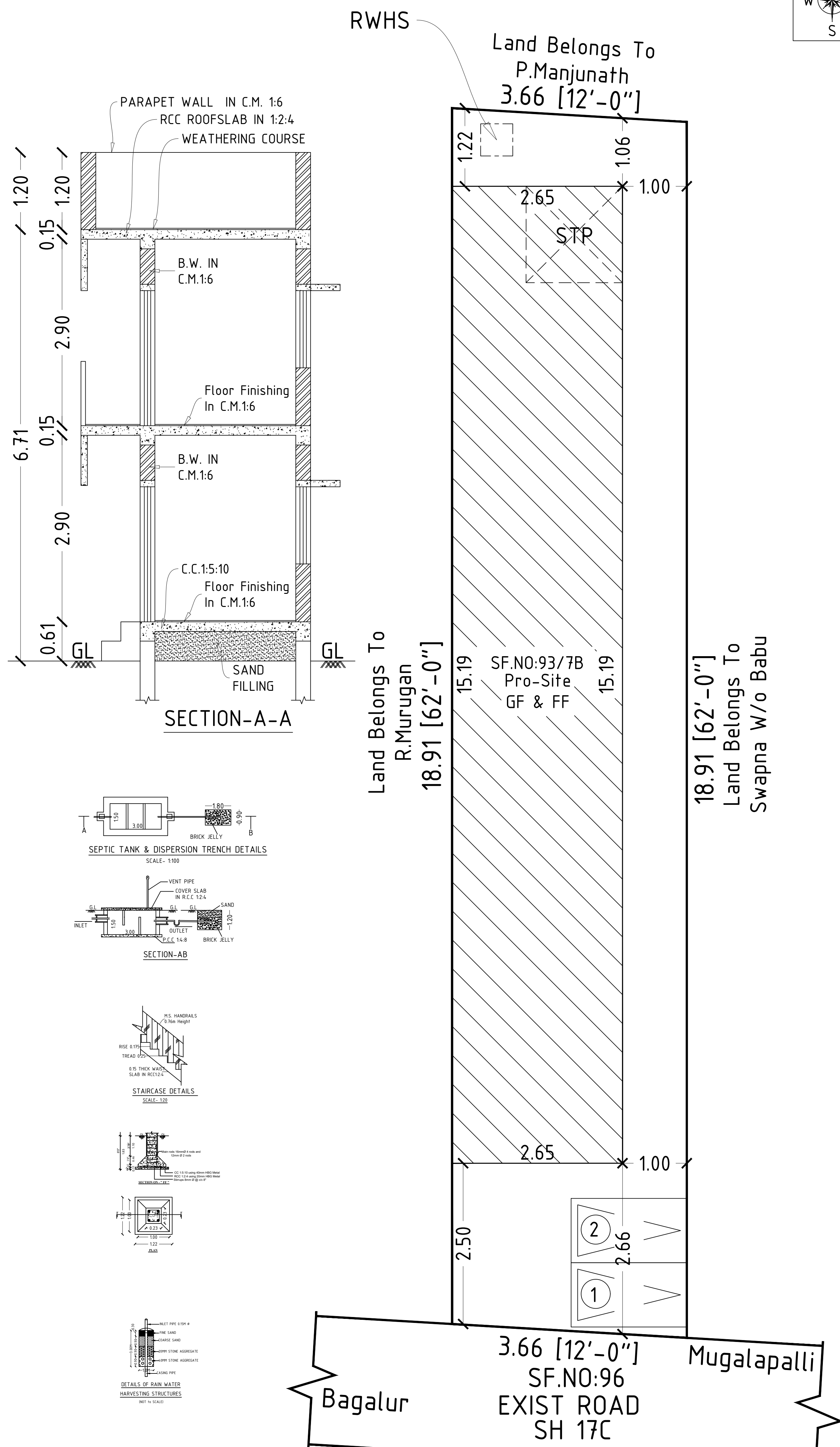
SITE PLAN
