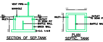
SECTION OF SEP.TANK
