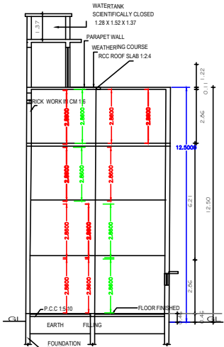
SECTION "A-B"
