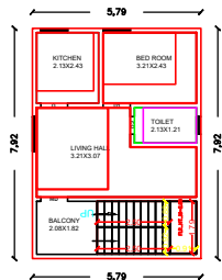
PRO. SECOND FLOOR PLAN.
