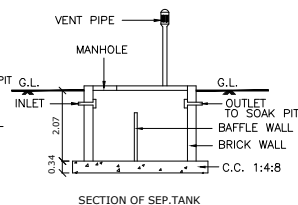
SECTION OF SEP.TANK
