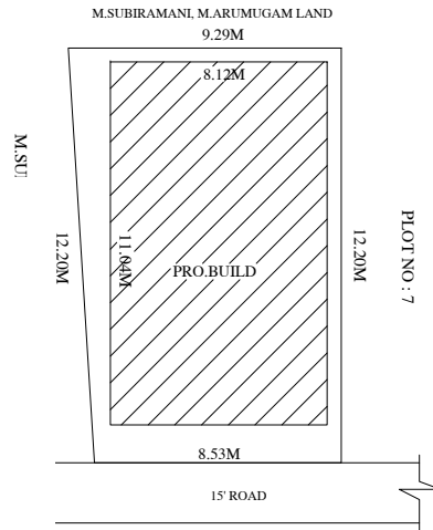
SITE PLAN
