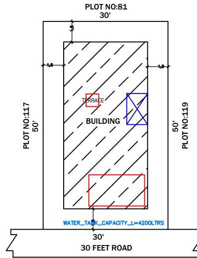
SITE PLAN
