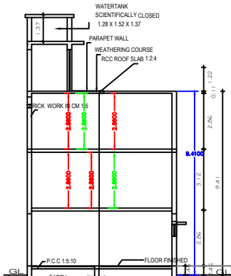
SECTION "A-B"
