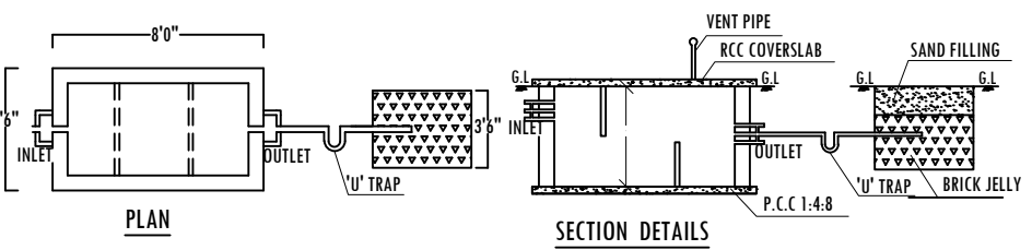
SEPTIC TANK AND DISPERSION TRENCH DETAILS
