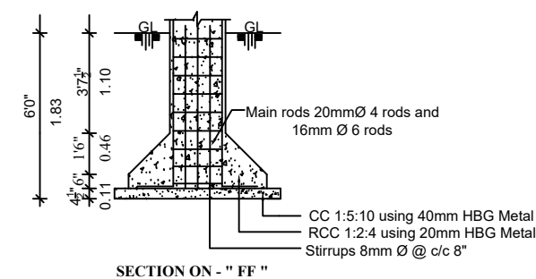
SECTION ON - " FF "
