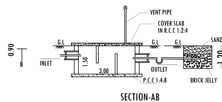
SECTION-AB
