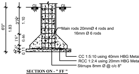
SECTION ON - " FF "
