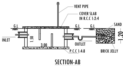
SECTION-AB
