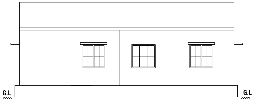
SIDE-ELEVATION
