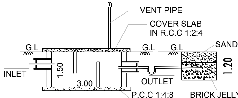
SECTION-AB
