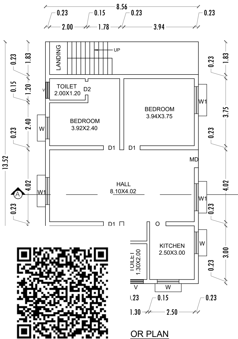
OR PLAN
