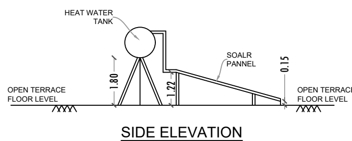
SIDE ELEVATION
