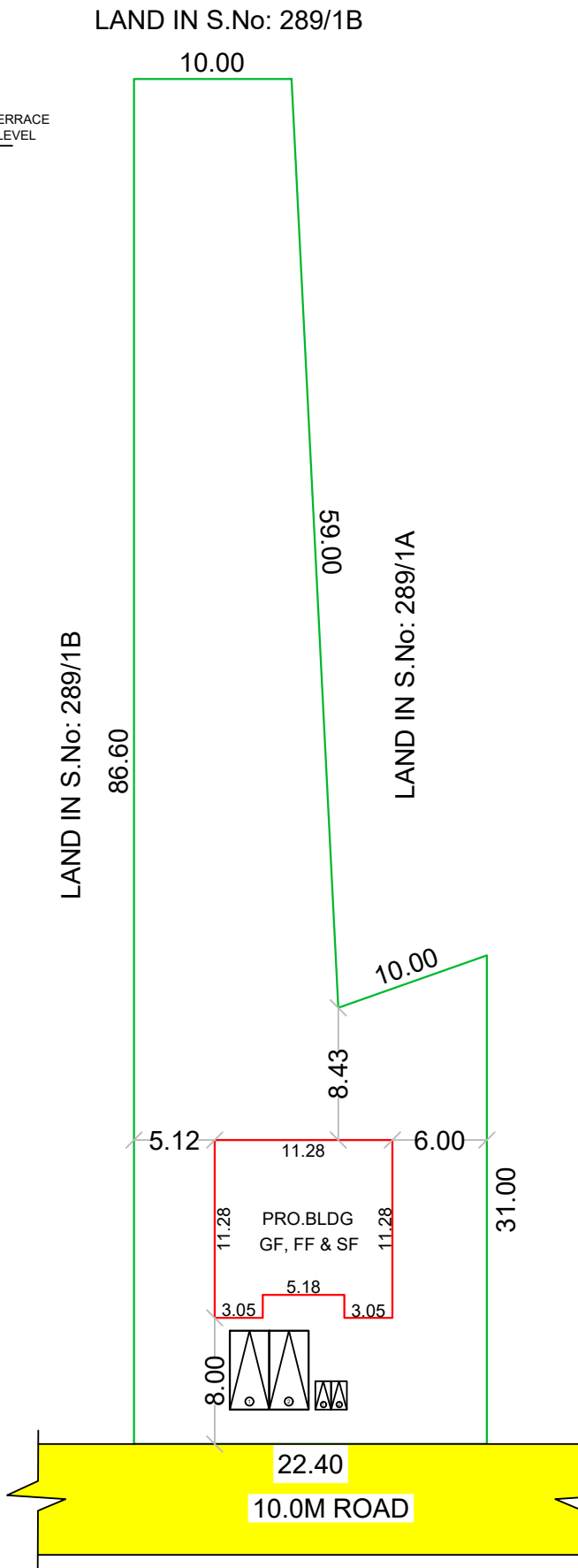
SITE PLAN
