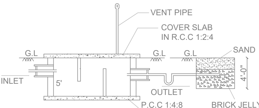
SECTION-AB
