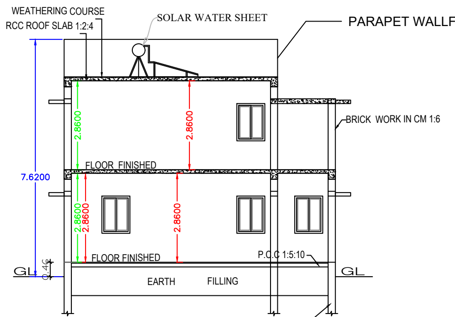
SECTION "A-B"
