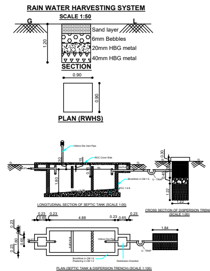
PLAN (SEPTIC TANK & DISPERSION TRENCH) (SCALE 1:10)
