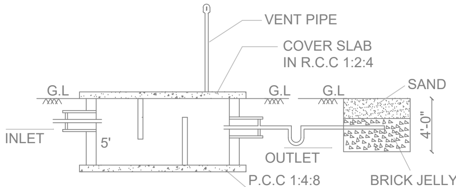
SECTION-AB
