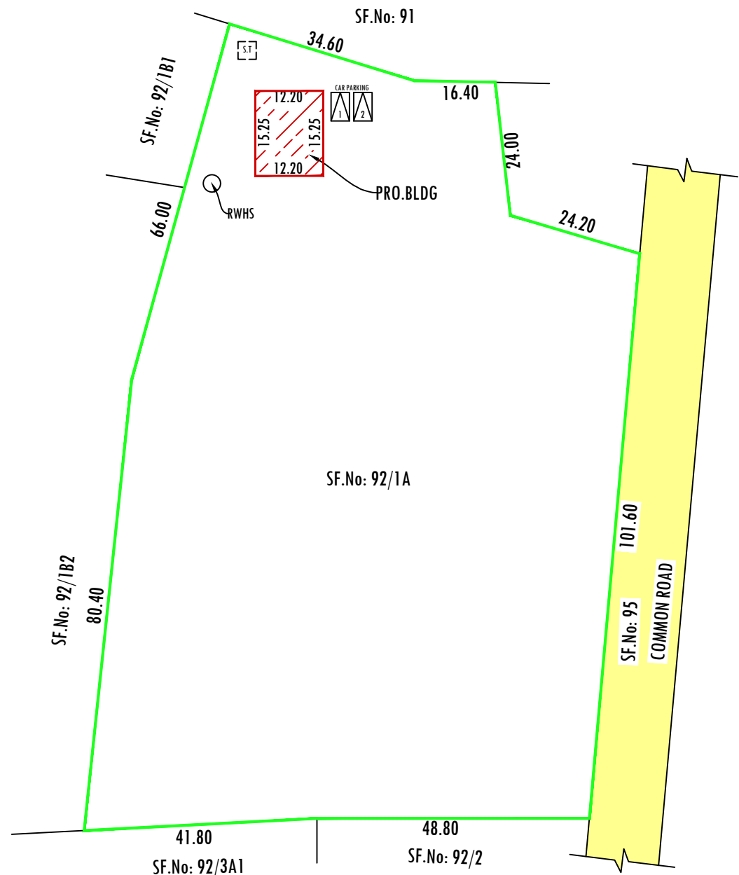
SITE PLAN SCALE- 1:800
