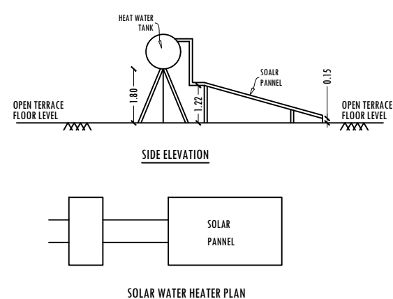
SOLAR WATER HEATER PLAN
