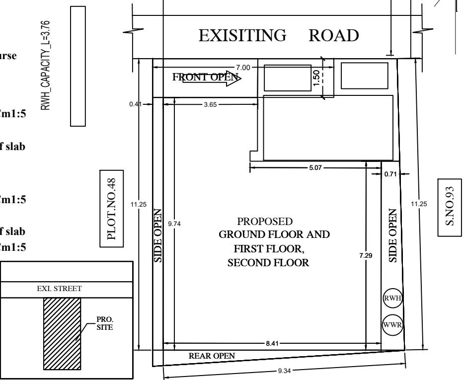
LOCATION PLAN
