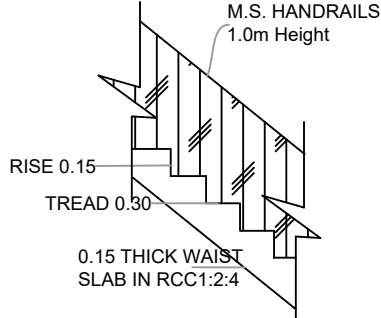
STAIRCASE DETAILS
