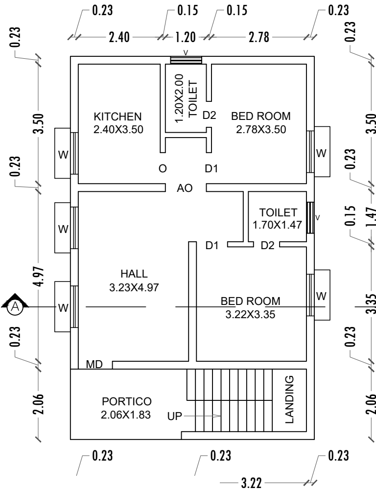
G.F. PLAN
