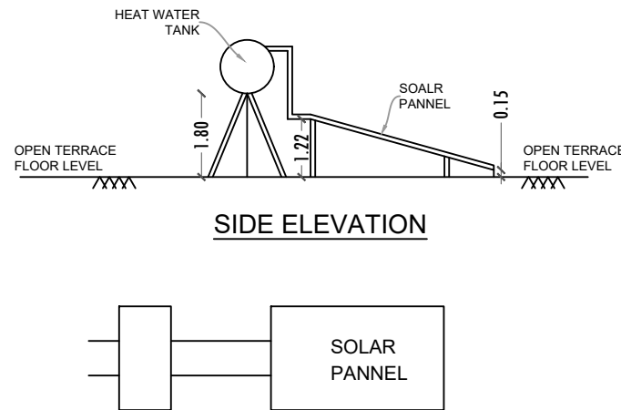
SOLAR WATER HEATER PLAN
