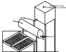
SOLAR SYSTEM (NOT TO SCALE)
