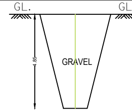
TRIAL PIT
