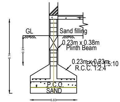
FOUNDATION DETAILS
