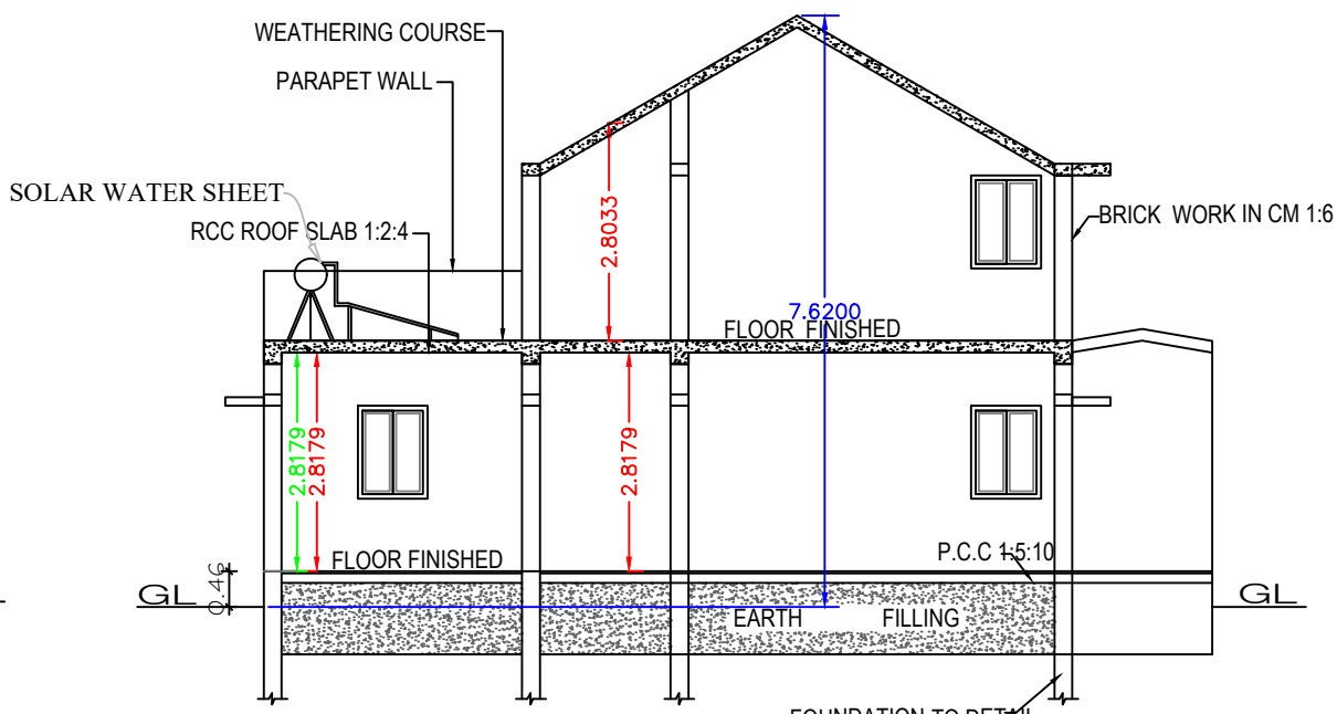
SECTION "A-B"
