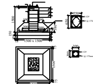
Foundation Details
