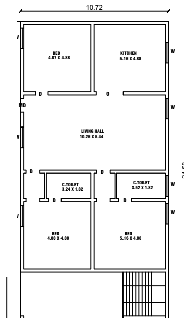
TYPICAL FIRST, SECOND & THIRD FLOOR PLAN
