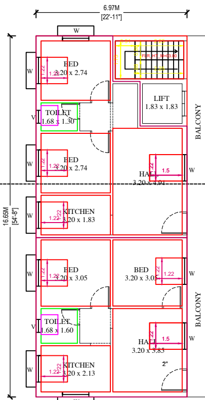
PRO.SECOND FLOOR PLAN
