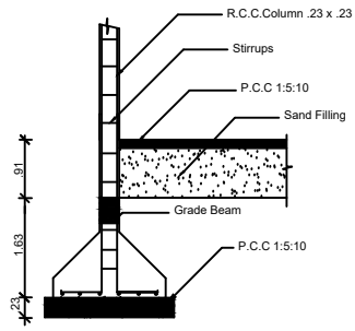
COLUMN DETAIL
