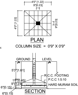
FOUNDATION DETAILS
