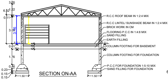
SECTION ON-AA
