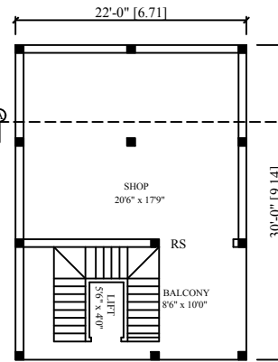
Pro-Second Floor Plan [1:100]
