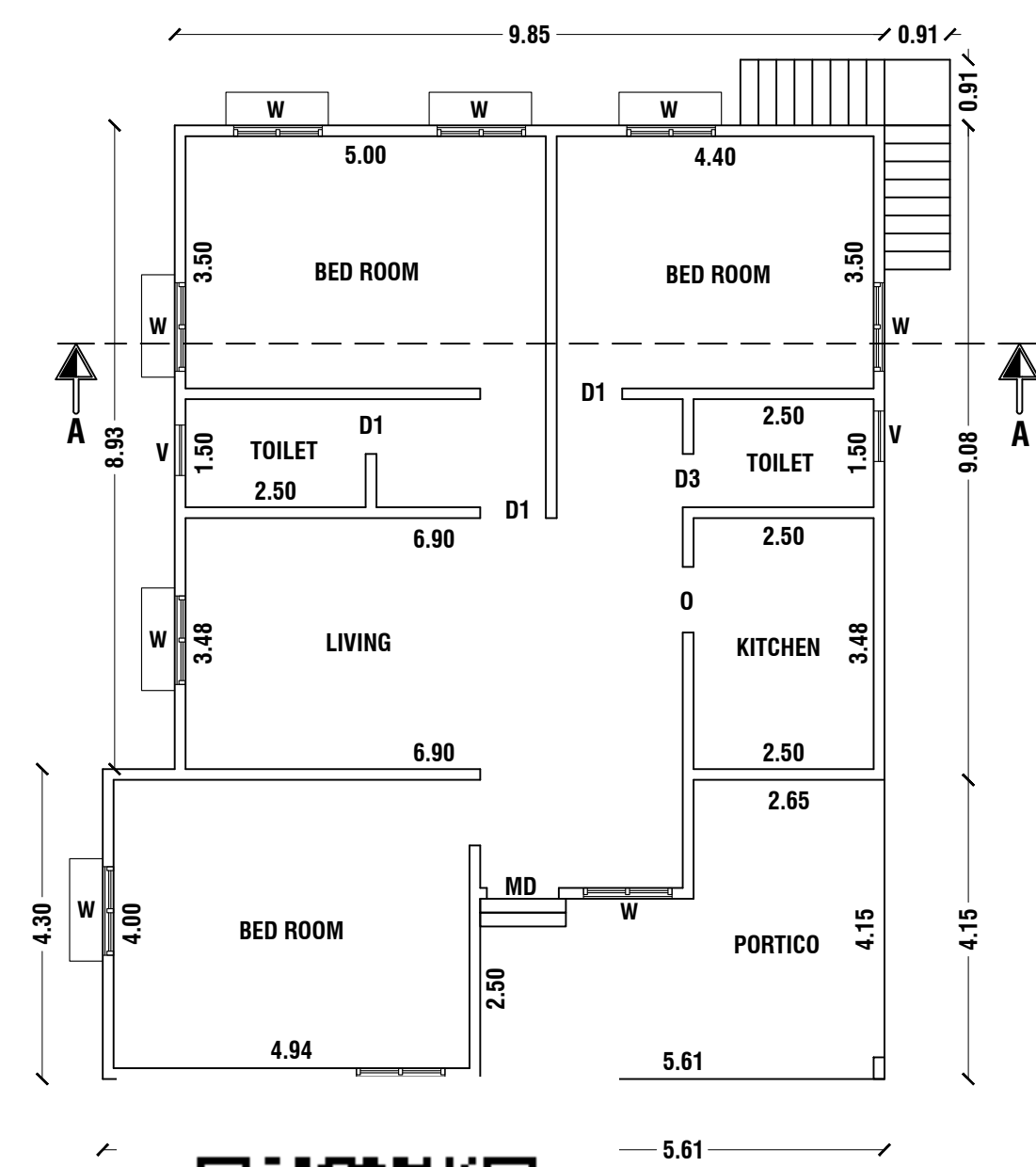
PLAN
