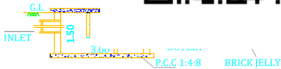
SECTION-AB
