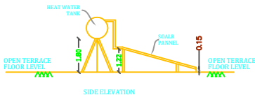
SIDE ELEVATION
