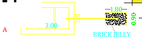
SEPTIC TANK & DISPERSION TRENCH DETAILS SCALE- 1:100
