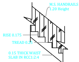
STAIRCASE DETAILS SCALE- 1:20
