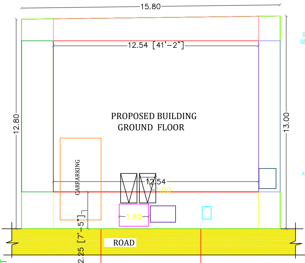
SITE PLAN
