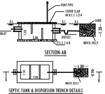
SEPTIC TANK & DISPERSION TRENCH DETAILS
