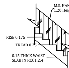
STAIRCASE DETAILS SCALE- 1:20
