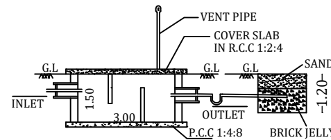
SECTION-AB
