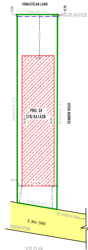
SITE PLAN SCALE 1:200
