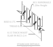
STAIRCASE DETAILS SCALE- 1:20
