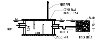
SECTION-AB
