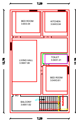
PRO. SECOND FLOOR PLAN.
