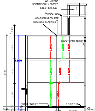
SECTION "A-B"
