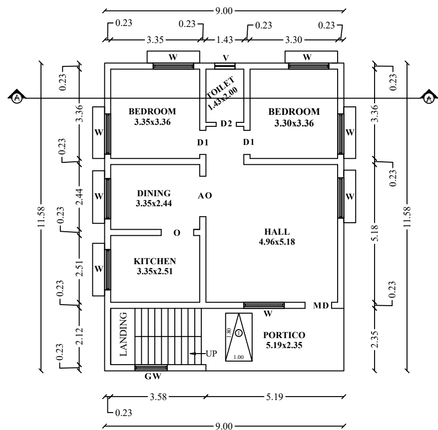
BLOCK - 1
