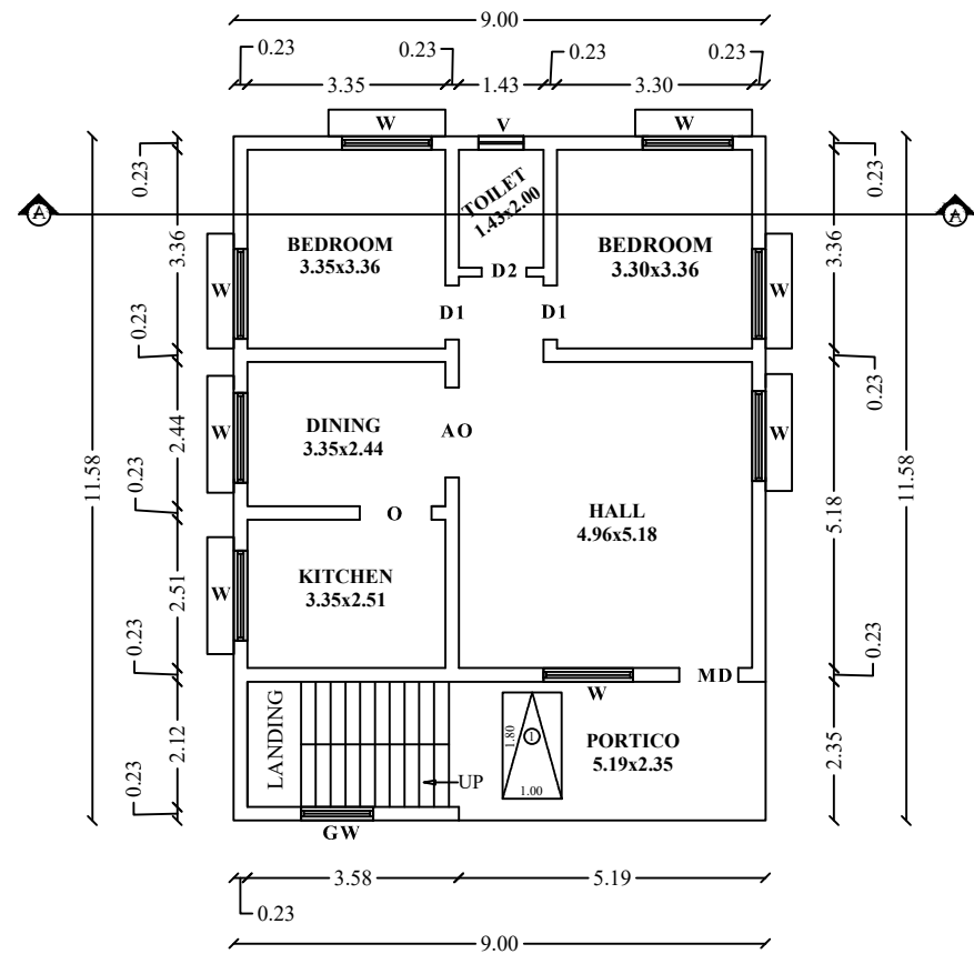
BLOCK - 2
