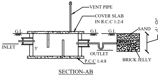
SECTION-AB
