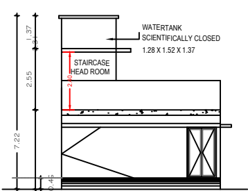
FRONT ELEVATION.
