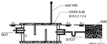
SECTION-AB
