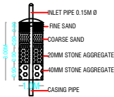
DETAILS OF RAIN WATER HARVESTING STRUCTURES
