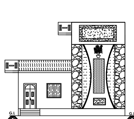
ELEVATION PLAN
