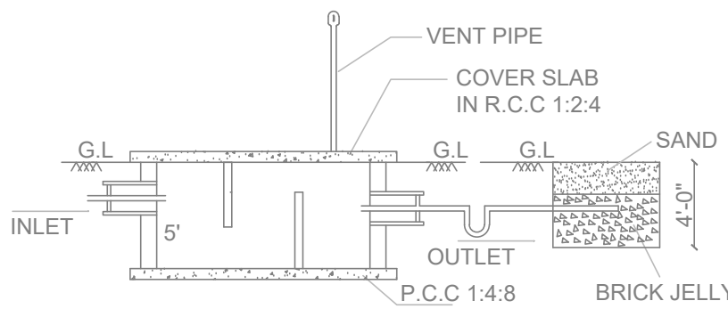
SECTION-AB
