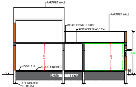
SECTION "A-B"
