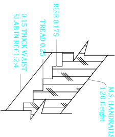
STAIRCASE DETAILS SCALE: 1/20
