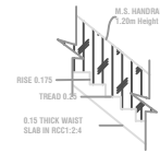
STAIRCASE DETAILS (NOT IN SCALE)
