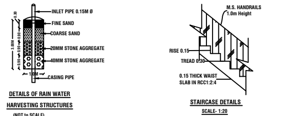
DETAILS OF RAIN WATER HARVESTING STRUCTURES (N.T.S.)
