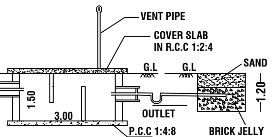
SECTION-AB
